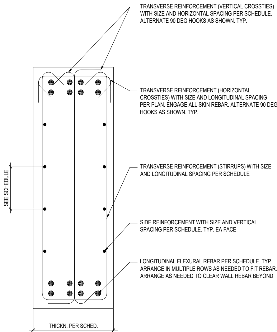
B2 SECTION
