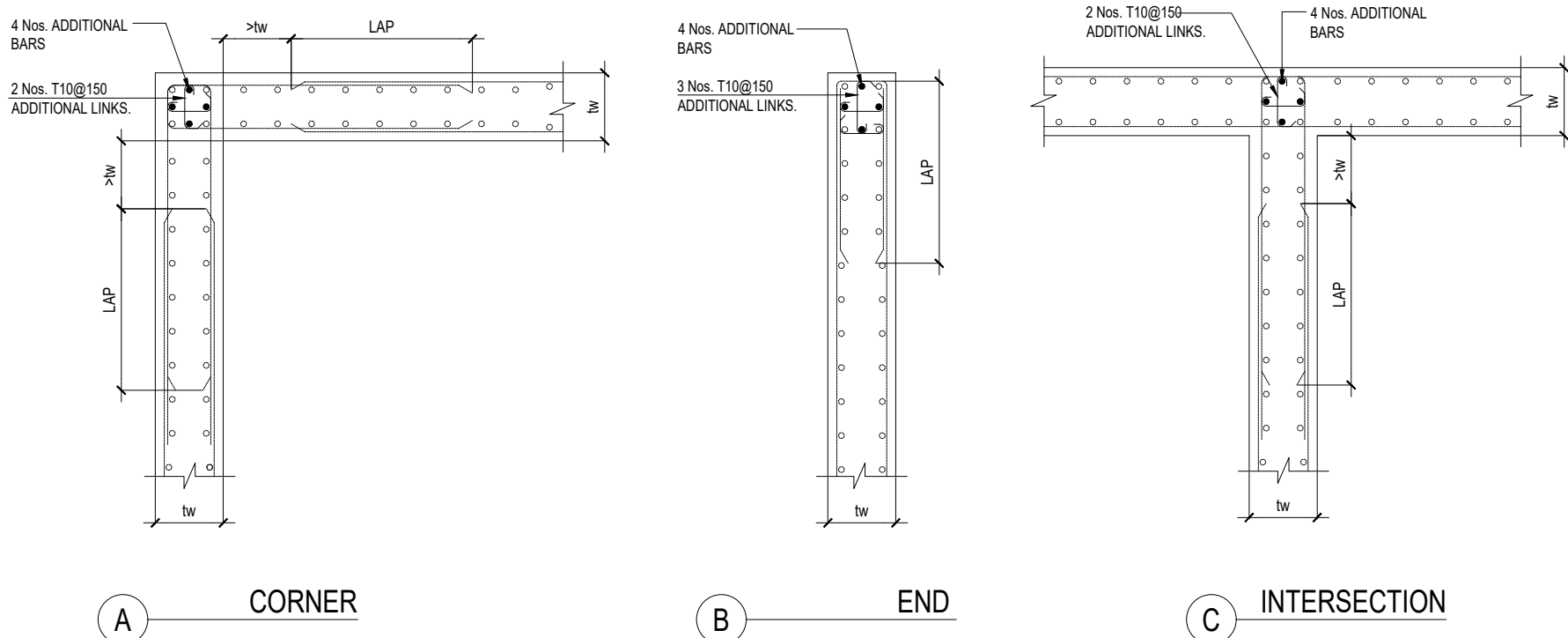
TYPICAL WALL JUNCTION DETAILS SCALE: N.T.S.
