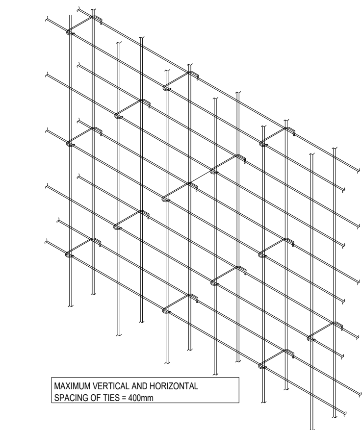
6 TYPICAL STAGGERED TIES IN WALLS SCALE: N.T.S.
